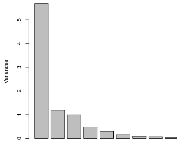
Screeplot, 9 principal components
